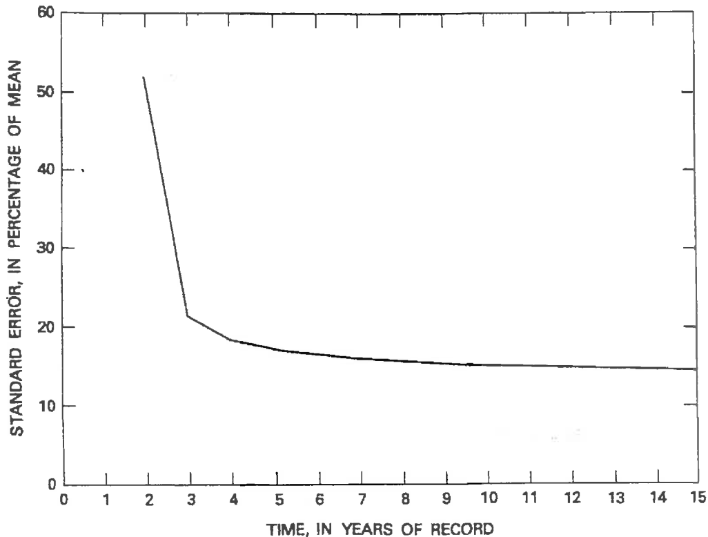
FIGURE 7.—Relationship of the standard error of estimate of low-flow correlations to varying years of record. Correlations are between September flows on Huntington Creek (09318000) and Ferron Creek (09316500).
